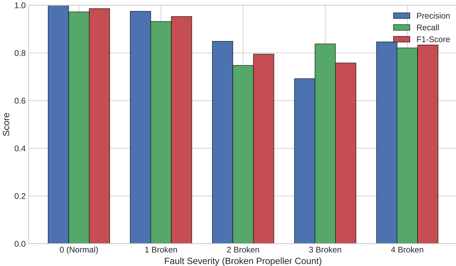
Per-Class Diagnostic Performance Breakdown
